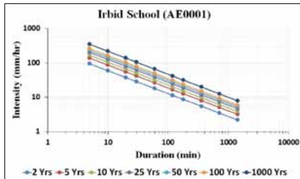
Figure 13. IDF Curve for Irbid School Station (Authours calculations).
