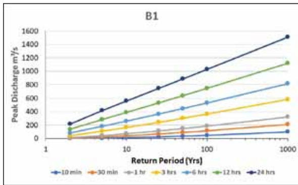
Figure 16. The peak discharge ( \text{m}^3/\text{s} ) in different durations and return periods in B1.
