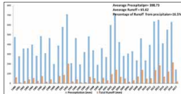
Figure 14. Annual precipitation and runoff, runoff percentage from Irbid School Station.
