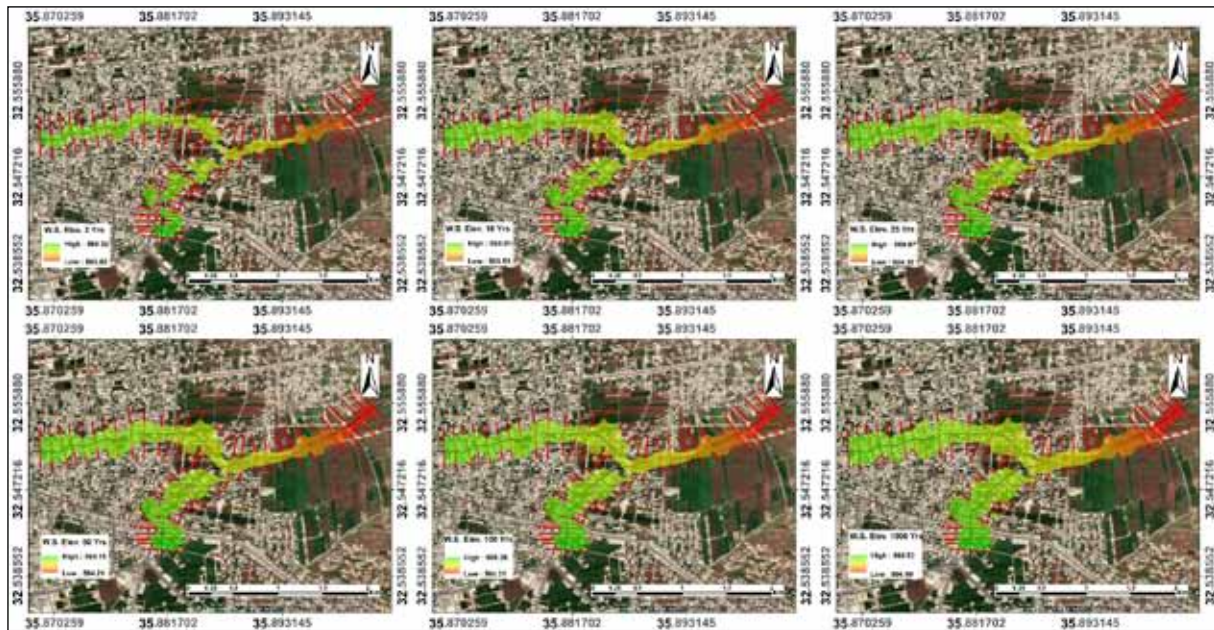
Figure 18. Flood inundation map, surface water elevation for Irbid (A) channel (return period 2, 10, 25, 50, 100, and 1000-Years).
