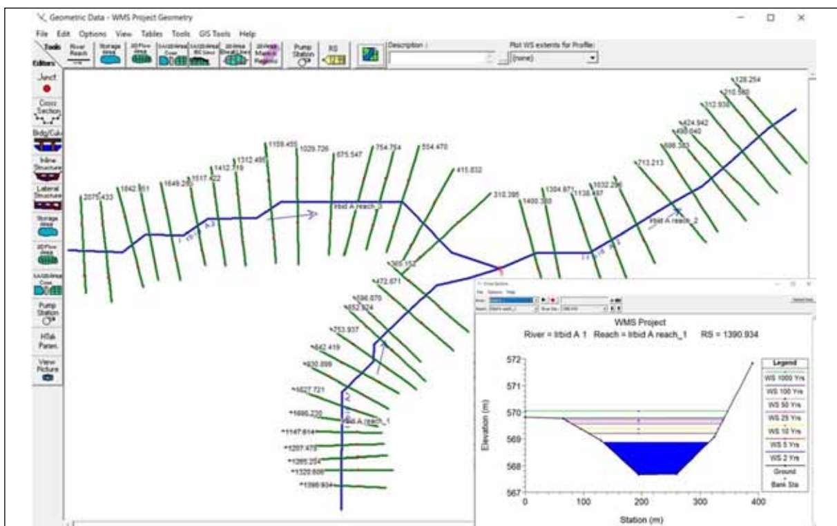
Figure 17. One of the channels and perpendicular cross sections in Irbid city (Irbid A channel).
