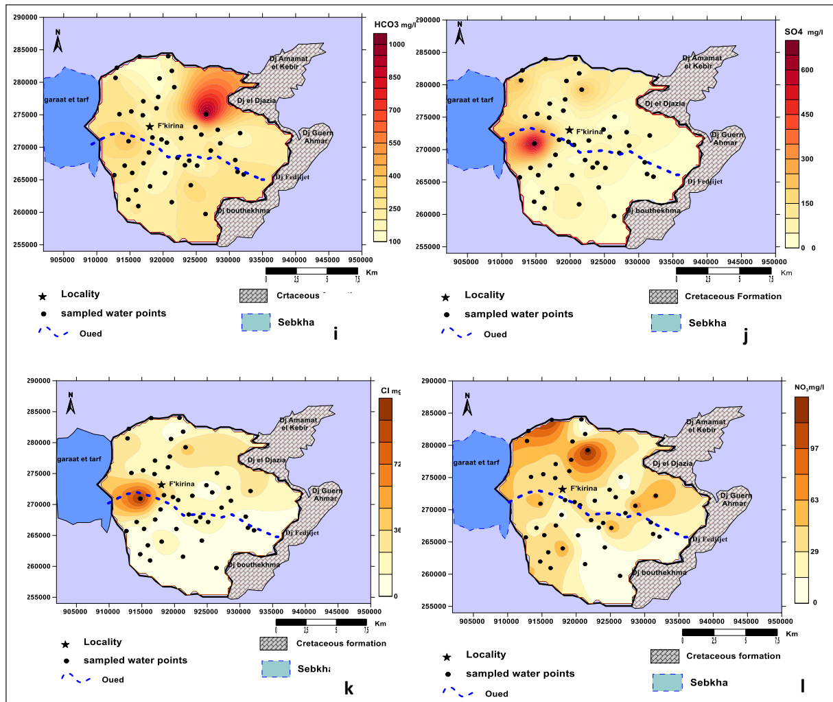
Figure 3. Map of F'kirina plain groundwaters for iso values of pH (a), EC (b), TDS (c), TH (d), Ca (e), Mg (f), Na (g), K (h), \text{HCO}_3^- (i), \text{SO}_4^{2-} (j), Cl (k), \text{NO}_3^- (l).
