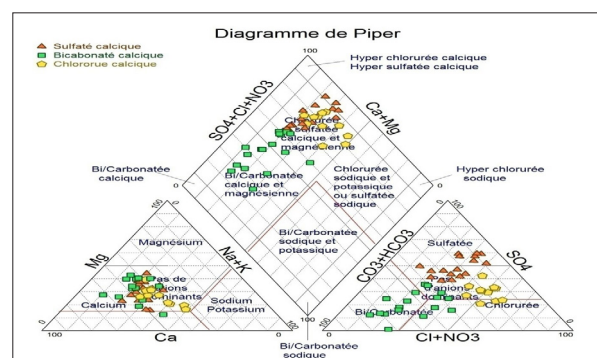
Figure 4. Piper diagram of the groundwater samples.
