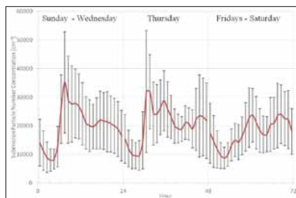
Figure 5. Daily patterns of the submicron particle number concentrations on three weekdays groups: (a) Sunday – Wednesday, (b) Thursday, and (c) Friday – Saturday.
