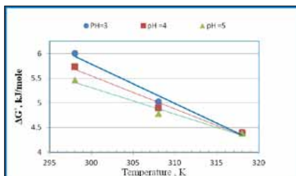
Figure 11. Relationship between temperature and \Delta G^\circ values at different temperatures and different pH values
