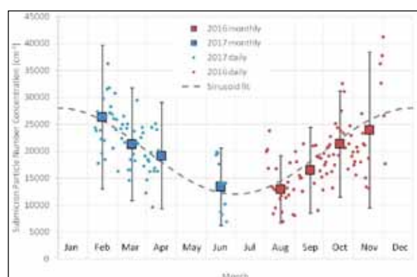
Figure 1. Seasonal variation of the submicron particle number concentrations fitted to a sinusoidal function of the form PN = 8 \times 10^3 \cos(360t/365) + 2 \times 10^4 , where PN is the particle number concentration [ \text{cm}^{-3} ], and t is the day of year starting from January 1 st .
