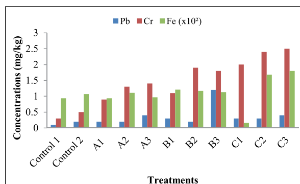
Figure 4. Heavy metal concentrations (August, 2016)
