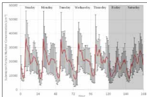
Figure 4. Weekly pattern of the submicron particle number concentrations.
