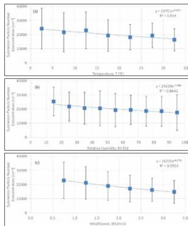
Figure 3. Submicron aerosol concentration versus the (a) temperature, (b) relative humidity, and (c) wind speed. These figures (average and standard deviation) were generated from the hourly average of the submicron particle number concentrations, and the trends were fitted to an exponential function.
