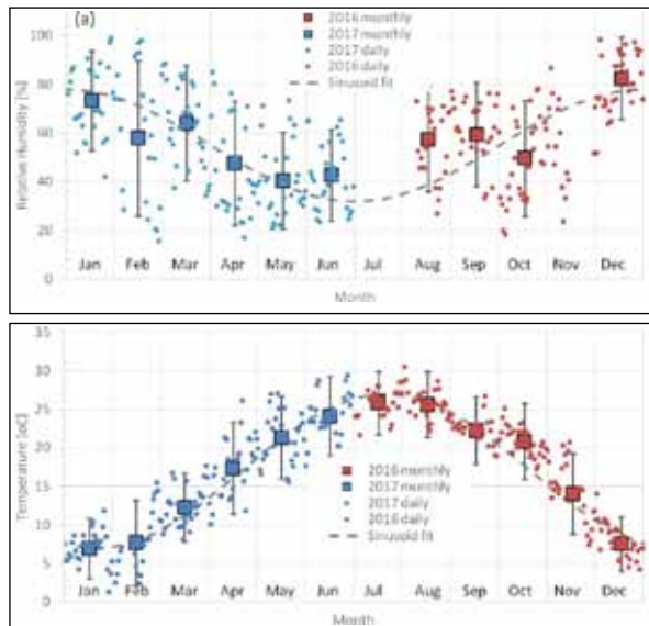
Figure 2. Seasonal variation of (a) relative humidity fitted to a sinusoidal function ( RH = 23 \cos(t/365 \cdot (^\circ 360^\circ)) + 55 , where RH is the relative humidity [%] and t is the day of year starting from January 1 st ) and (b) temperature fitted to a sinusoidal function ( T = 10 \sin(360(t - 112)/365) + 17 , where T is the Temperature [°C] and t is again the day of year).
