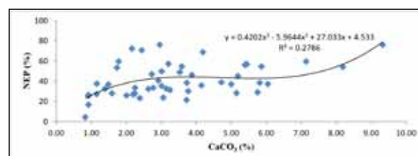
Figure 4. Mean non-erodible soil particles (NEP) versus \text{CaCO}_3 content
