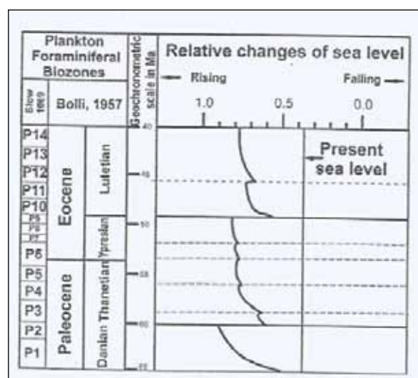
Figure 6. The Ypresian/Lutetian boundary relative to the global sea level fluctuation of Vail et al. (1977).
