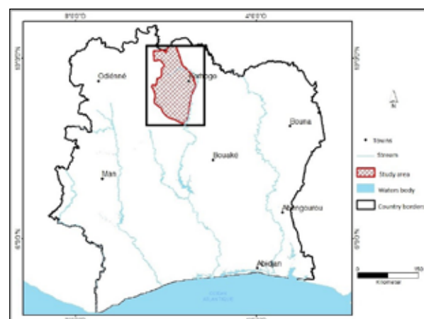
Figure 1. Study area located at (9° 27' to 9° 57' N; 5° 39' to 5° 58' W) in the northwest of Ivory Coast.
