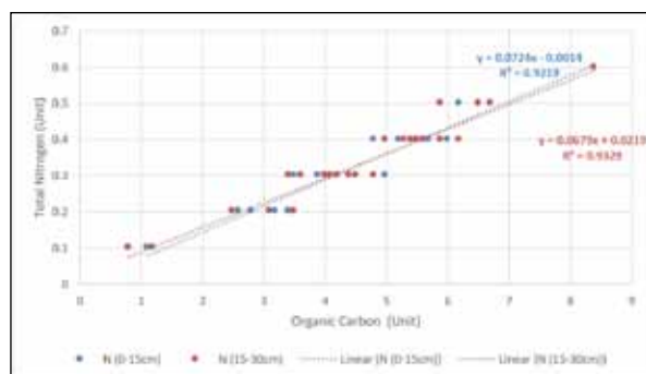
Figure 8. The study area (Odeda LGA) showing the linear regression between Nitrogen and Organic Carbon.
