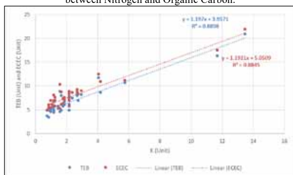
Figure 9. The study area (Odeda LGA) showing the linear regression among K versus TEB/ECEC.
