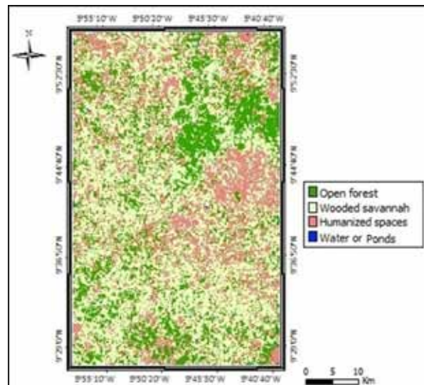
Figure 7. Result of the classification of the land cover of the study area in 2019.
