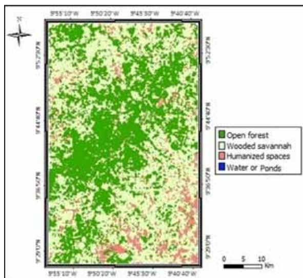
Figure 5. Result of the classification of the land cover of the study area in 1986.
