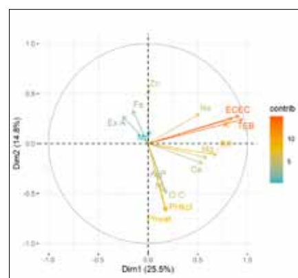
Figure 7. Variable factor map of Principal component analysis for soil sampled at 0 - 15cm depth.
