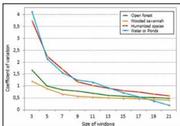
Figure 3. Coefficient of variation of the contrast parameter (Sentinel-2 of February 12, 2019).
