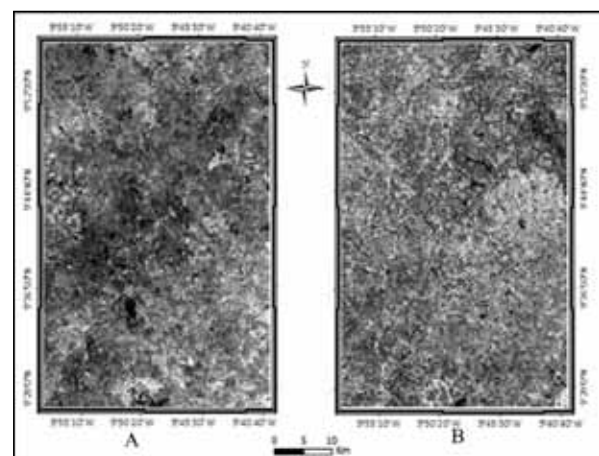
Figure 4. Result of the ACP transformation. A) Main component1 (Landsat TM, January 16, 1986); B) Main component1 (Sentinel-2, February 12, 2019).
