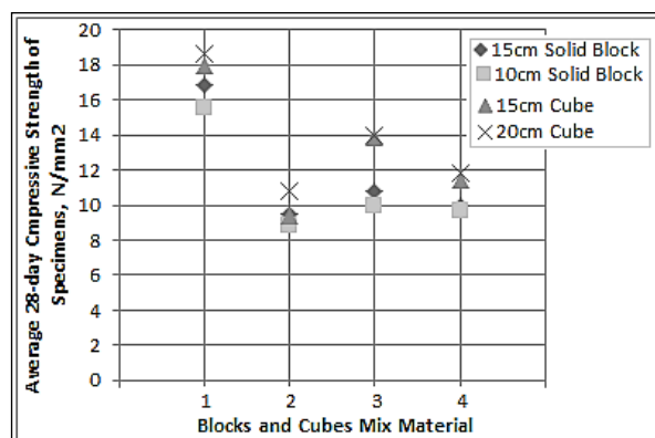
Figure 4. Compressive strength of block material: Mix #1: Ordinary Materials, Mix #2: Pozolanic Addasyah, Mix #3: Pozolanic Swailah, and Mix #4: Pozolanic Boudrah.
