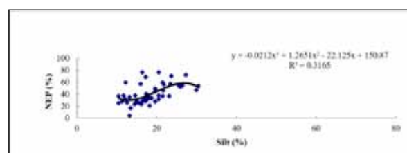
Figure 2. Mean non-erodible soil particles (NEP) versus silt content
