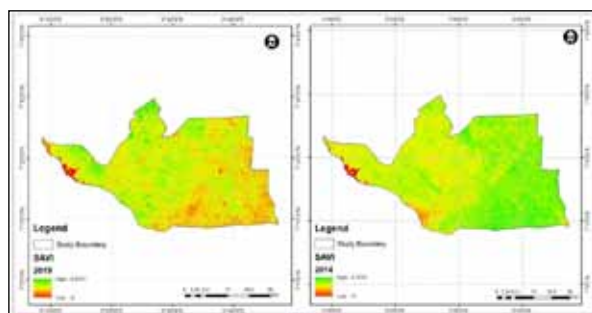
Figure 6. The study area (Odeda LGA) showing the year 2014 and 2019 soil adjusted the Vegetation index.
