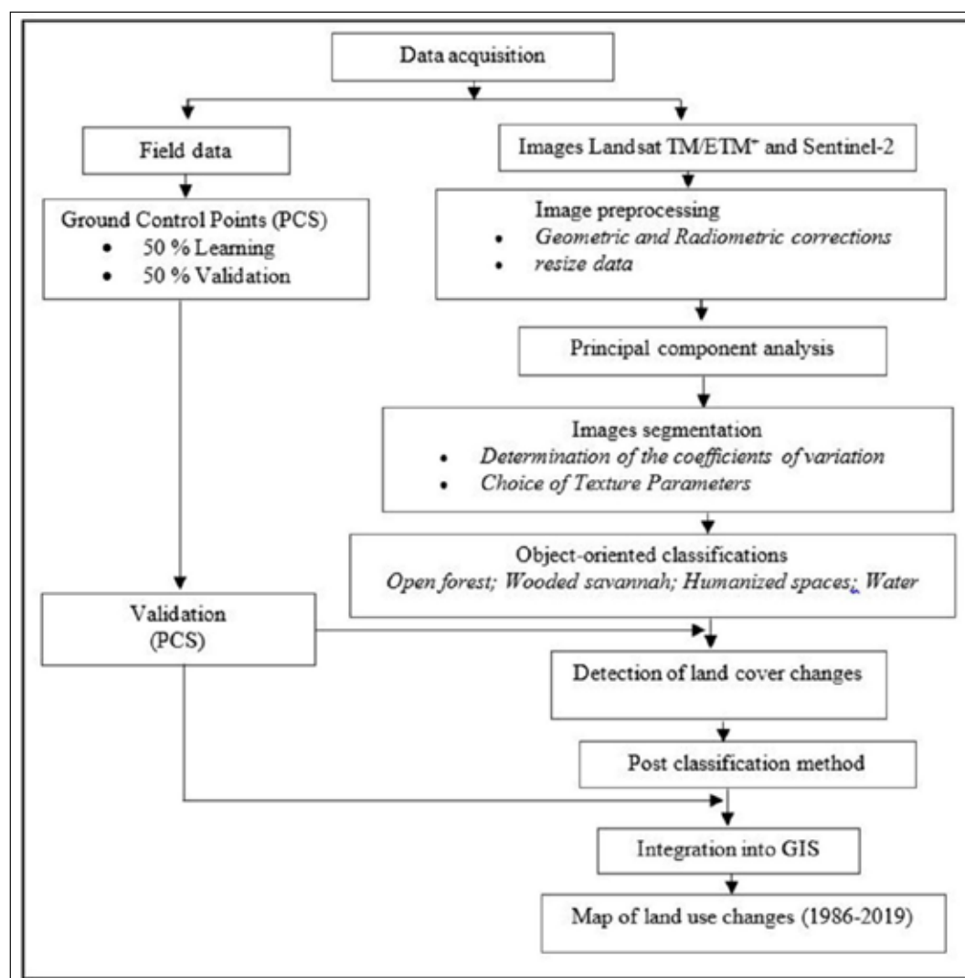
Figure 2. Methodological flowchart of monitoring and detecting land-use changes in the department of Korhogo.
