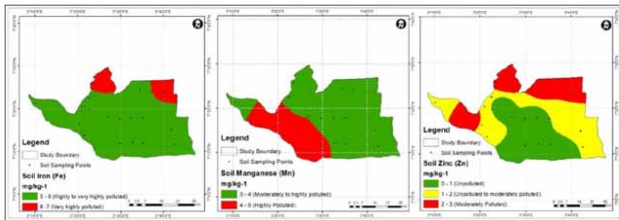
Figure 12. The study area (Odeda LGA) showing the Geoconcentration of soil iron, manganese, and zinc.
