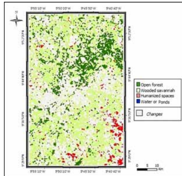
Figure 8. Global map of changes (1986-2019).
