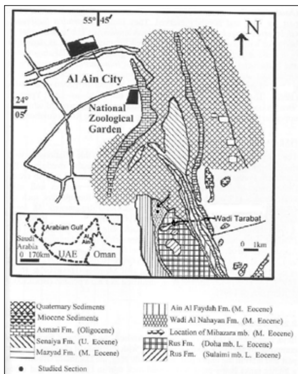
Figure 3. Geologic map of Jabal Hafit (UAE) including the study section of the Middle Eocene Wadi Al Nahayan Member of the Dammam Formation (after Hamdan and Bahr, 1992) outcropping at the western limb of Jabal Hafit (after Boukhary et al., 2006).
