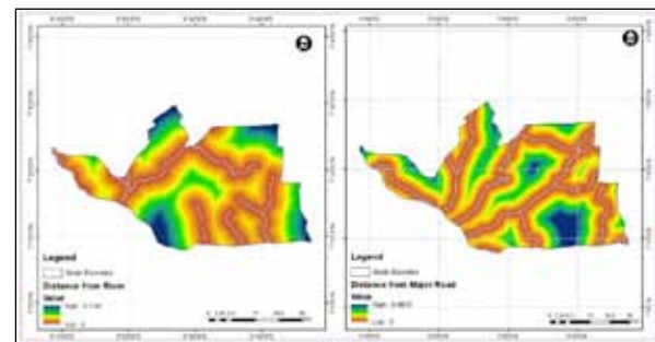
Figure 2a. The study area (Odeda LGA) showing the distance from Major Road and River.
