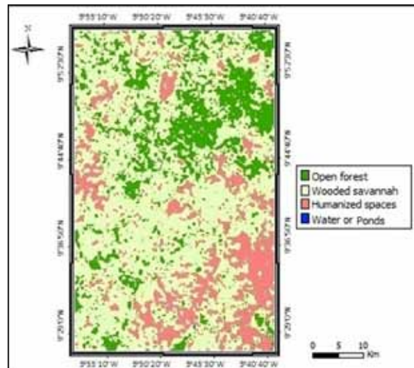
Figure 6. Result of the classification of the land cover of the study area in 2002.
