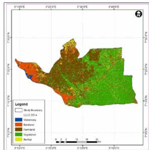
Figure 3. The study area (Odeda LGA) showing the year 2014 LULC changes.
