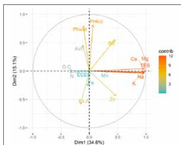
Figure 11. The study area (Odeda LGA) showing the variable factor map of principal component analysis for soil samples at 15-30 cm.
