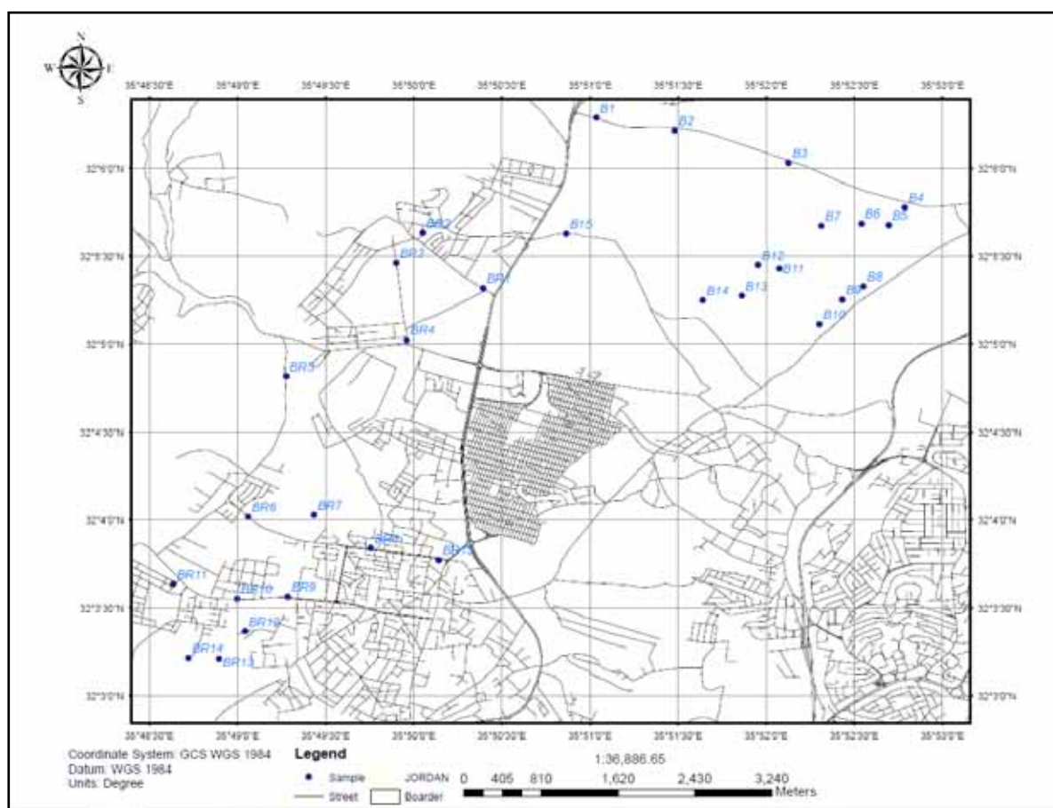
Figure 3. The map shows the sample location.
