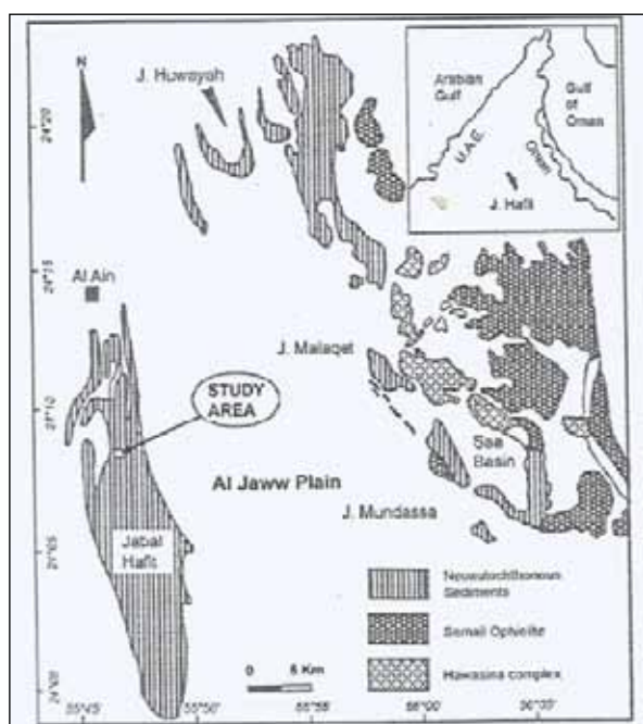
Figure 1. Location map of Al Ain area, UAE including Jabal Hafit (west of Al Jaww Plain), J. Malaqet and J. Mundassa, east Al Jaww Plain (after Anan, 2015a).
