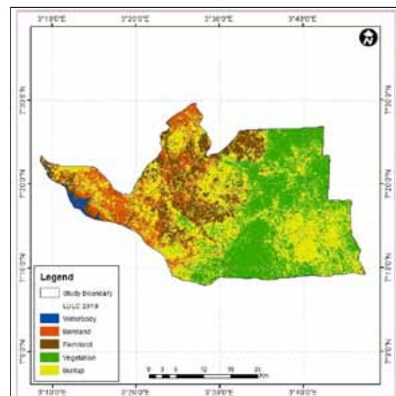
Figure 4. The study area (Odeda LGA) showing the year 2019 LULC changes.
