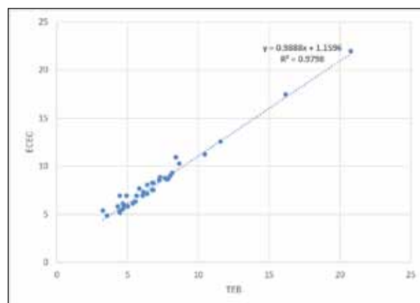
Figure 10. The study area (Odeda LGA) showing the linear regression between TEB and ECEC.
