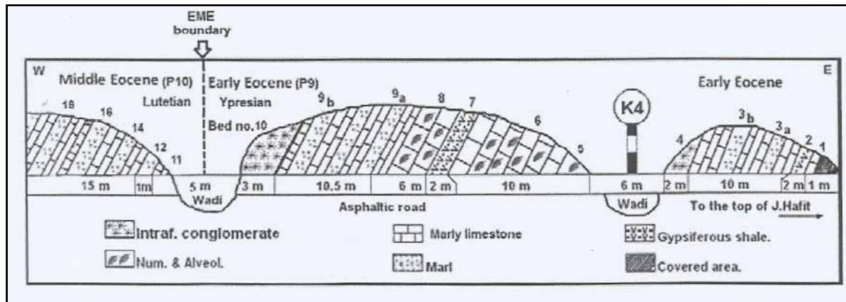
Figure 2. Schematic section of the Early/Middle Eocene succession at K4 of J. Hafit (after Anan, 2015a).
