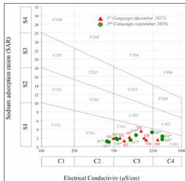
Figure 5. Irrigation water suitability of Guenitra watershed according to Richards (1954).
