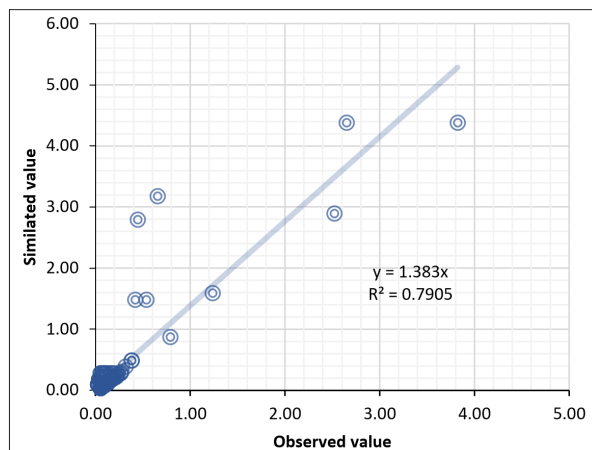
Figure 10. Comparison of simulated discharge and observed runoff in the Wadi Laussif subbasin
