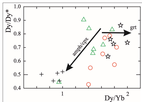
Figure 10. The Dy/Dy^* vs. Dy/Yb plot (Davidson et al., 2013). The arrow indicated by the garnet might indicate the amount of residual garnet in the source area of Sabil granodiorite.
