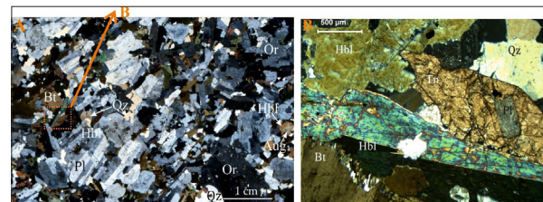
Figure 6. A. whole thin section microphotograph of Sabil granodiorite (X-Nicols, Sample NF-8). Flow texture is well demonstrated by the twinned prismatic oligoclase (PL). Hornblende (Hbl., biotite (Bt.), and titanite (Tn) form clusters. Some hornblende is rimming augite (Aug). Orthoclase (Or) and quartz (Qz) are interstitial phases. B. Enlarged part of A, indicated by the arrow, showing hornblende, titanite quartz, and biotite.
