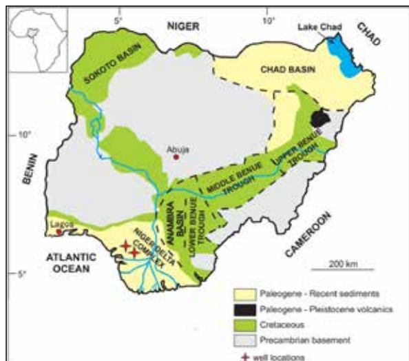
Figure 1. Simplified geologic map of the Niger Delta Basin indicating the well locations (Obaje, 2009).
