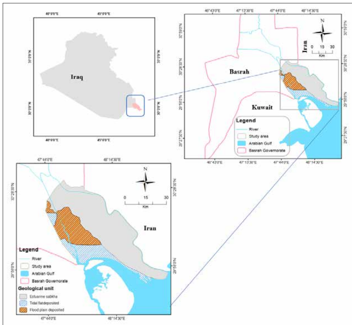
Figure 1. Location of the study area with the geological 'unit' map.
