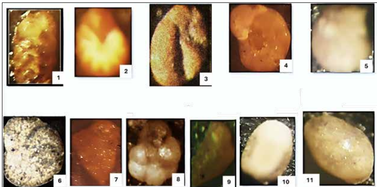
Plate 1. Photos of some selected foraminifera and miscellaneous microfossils (Holothuroidea and Ostracoda) from both wells.
