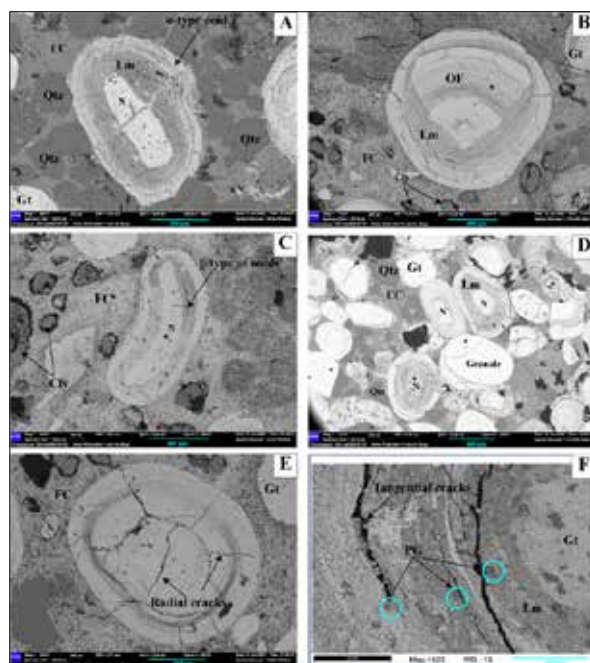
Figure 6. SEM images of Aïn Babouche ooidal ironstones. a) \alpha -type of ooid with quartz grains and carbonate cement in Djebel Dahar ironstones. b) Ooid fragment as nucleus and clay grains cemented with a ferruginous cement in Kef en Nsour ironstones. c) \beta -type ooid with clay grains cemented with a ferruginous cement in Kef en Nsour ironstones. d) Ooids, granules, and quartz cemented with carbonate cement in Djebel Dahar ironstones. e) Ooid represents the radial type of cracks in Kef en Nsour ironstones f) The concentric layers of ooid contain phosphate grains. (Lm: limonite. Gt: Goethite Qtz: quartz. Ap: Apatite. Cly: Clay. PG: Phosphate grains. N: nucleus. CC: carbonate cement. FC: ferruginous cement. OF: ooid fragment)
