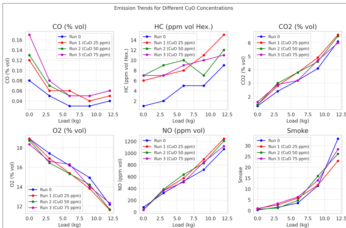
Figure 6. Comparative analysis of emission parameters for neat diesel (Run 0) and CuO nanoparticle blends (25, 50, and 75 ppm)
