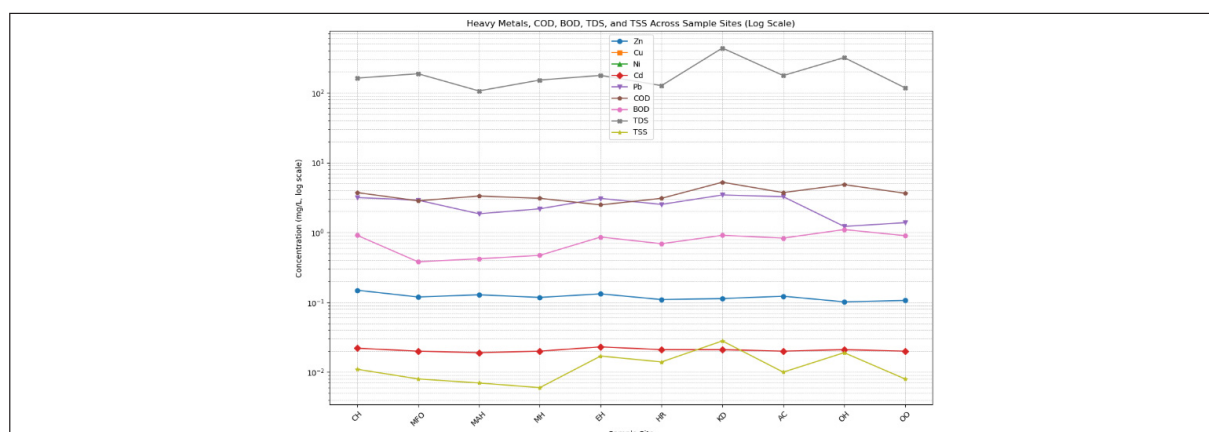
Figure 2. Line graph Showing the Concentrations of heavy metals and physicochemical parameters in the study Area.
